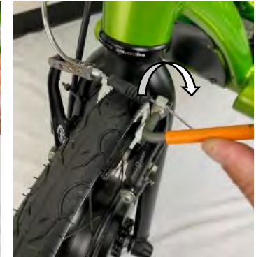
Tighten cable pinch bolt
